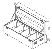
Flight Case (1320400095)
